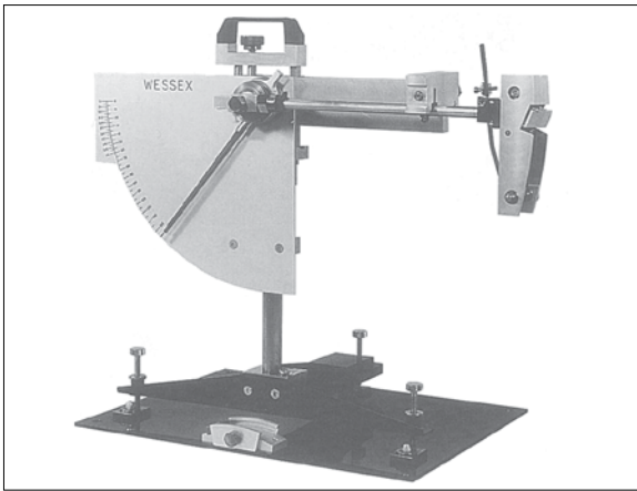
Figure 4. A British Pendulum Tester
