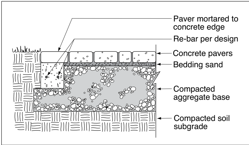
Figure 8. Submerged concrete edge.
