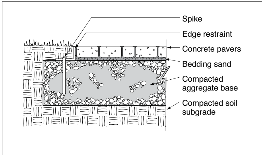
Figure 5. Aluminum edging.
