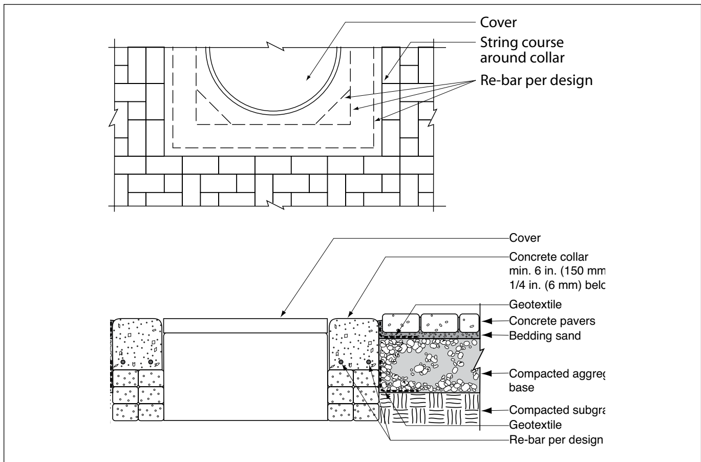
Figure 9. Utility cover.
