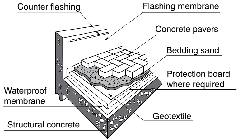
Figure 3. Roof assembly
