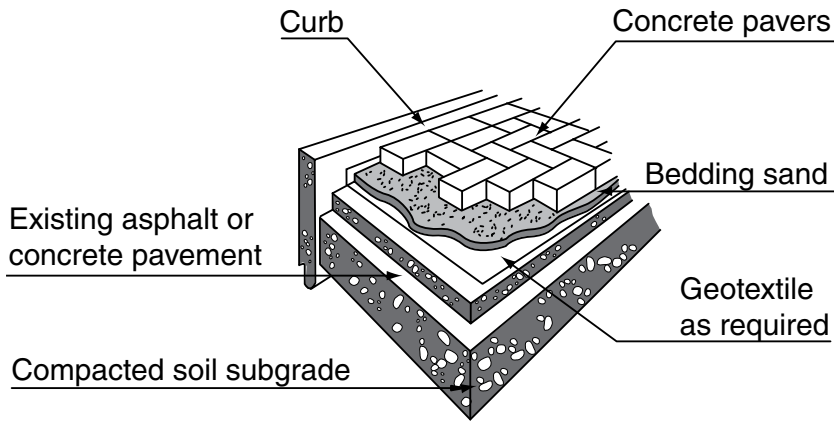
Figure 5. Typical overlay/inlay on existing pavement.
