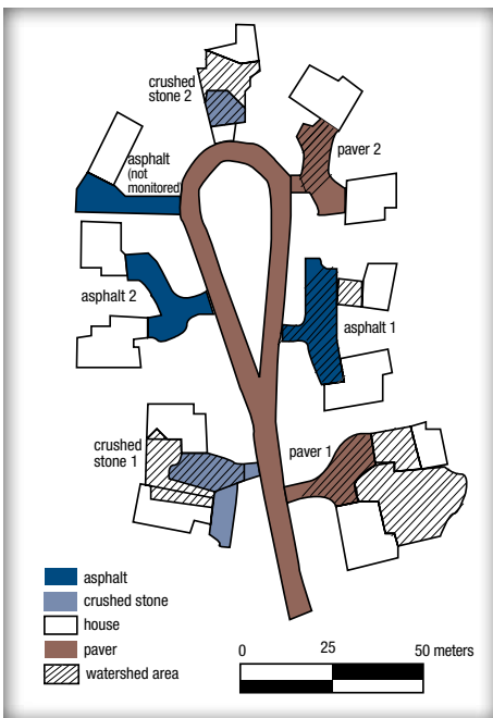
Runoff from various types of pavements are being monitored in the Glen Brook Green Subdivision in Waterford, Connecticut.
