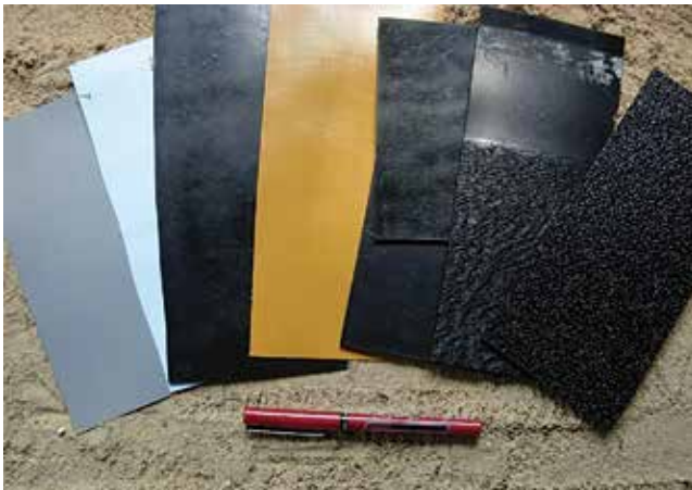
Figure 4. Geomembrane examples
