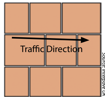
Figure 22. Longitudinal Running Bond
