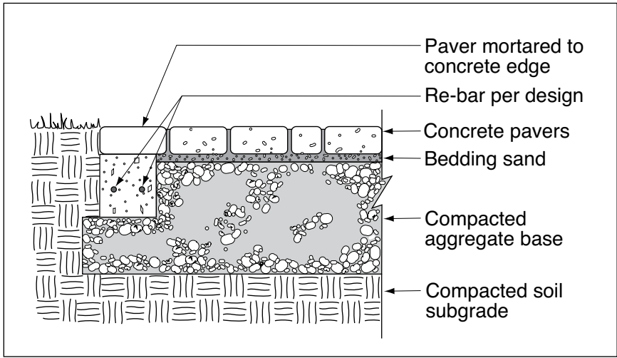
Figure 8. Submerged concrete edge.
