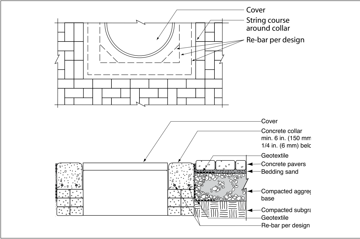
Figure 9. Utility cover.
